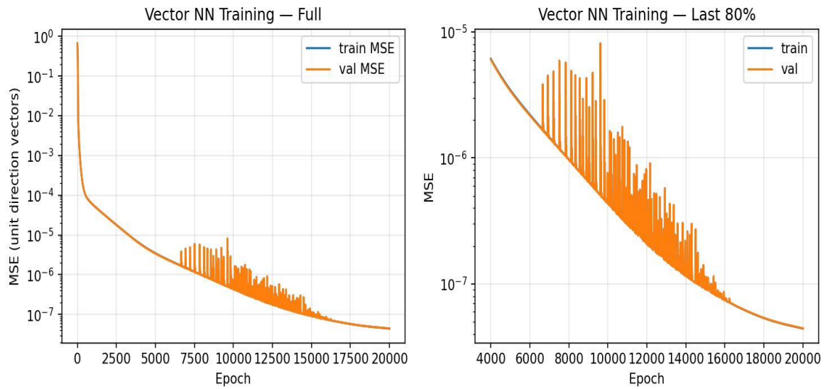
Figure 1. Vector NN training curve over 20,000 epochs. Left: full run (log scale). Right: last 80% confirming convergence. Val MSE = 4 \times 10^{-7} at epoch 20,000.
